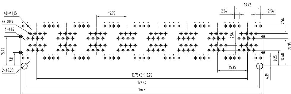
PC Board Layout Component Side Shown
